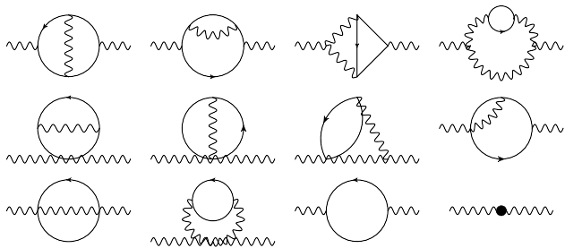
Figure: Diagrams contributing to the graviton self-energy. The filled circle corresponds to the cosmological constant term. Wiggly and solid lines represent the graviton and the matter field propagators, respectively.
